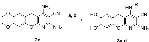
Scheme 4. Reagents and conditions: (a) NaOH, DMSO, R-Br; (b) BBr 3 /DMSO.
