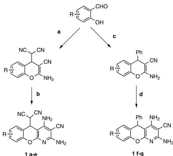
Scheme 1. Reagents and conditions: (a) CH 2 (CN) 2 (2 equiv), cat. piperidine/EtOH, rt; (b) CH 2 (CN) 2 , cat. piperidine/EtOH, reflux; (c) Ph–C=C(CN) 2 , cat. piperidine, EtOH, reflux; (d) CH 2 (CN) 2 , pyridine, reflux.
