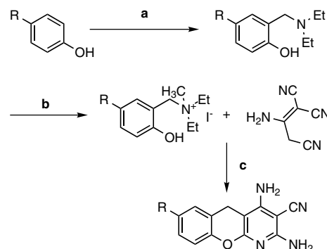
Scheme 2. Reagents and conditions: (a) Et 2 NH, CH 2 O; (b) CH 3 I/acetone; (c) EtOH, cat. piperidine, heat.
